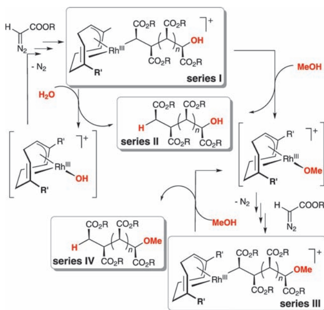
Scheme 3. Reaction mechanism showing series I–IV ( R' = \text{H}, \text{Me} , R = \text{Et}, \text{Bn} ).
